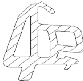
Joint HI
